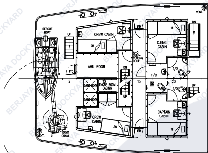
BOAT DECK PLAN
