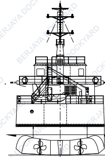
STERN VIEW
