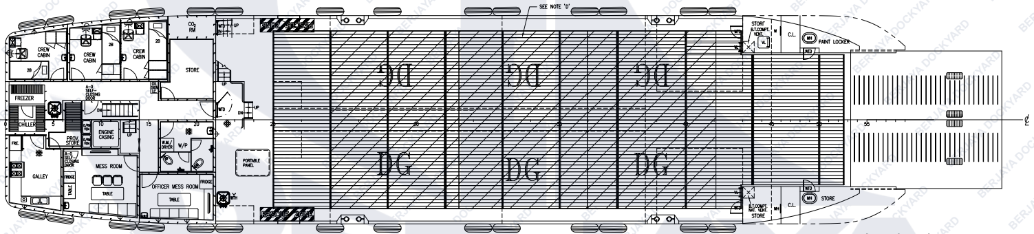
MAIN DECK PLAN
