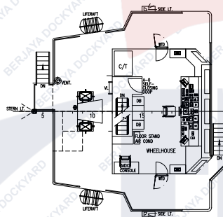
NAV. BRIDGE DECK PLAN
