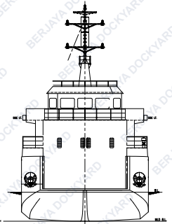
FWD VIEW
